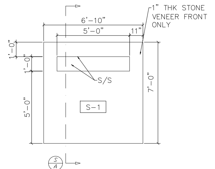
CENTER WALL ELEVATION
